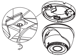
Figure 2-3 Install the Turret Camera
