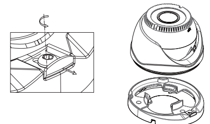
Figure 2-2 Remove the Clip Plate
