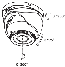
Figure 2-4 3-axis Adjustment
